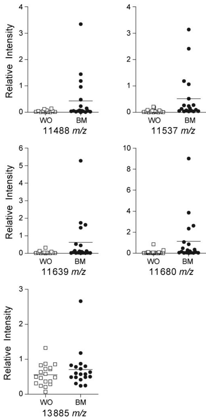
Fig. 2. Scatter plots of peak intensities for the four peaks of interest. Biological replicates with the mean intensities of the four peaks in serum samples from patients with bone metastasis (BM) that were found to be statistically significantly increased [ m/z 11 488 ( P = 0.0020 ); m/z 11 537 ( P = 0.0004 ); m/z 11 639 ( P = 0.0022 ); m/z 11 680 ( P = 0.0051 )]. A plot of the peak intensities of the neighboring statistically insignificant ( P = 0.3812 ) m/z 13 885 peak (bottom panel) is included for reference. WO, patients without bone metastases.
