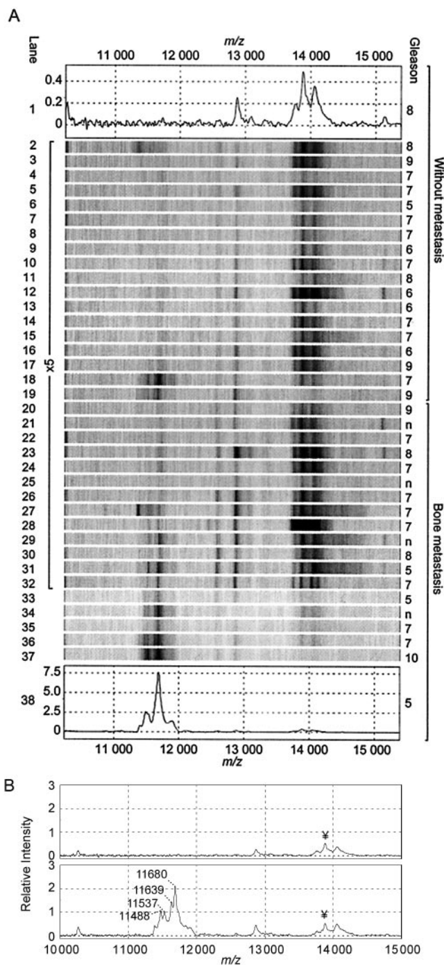
Fig. 1. SELDI-TOF MS spectra of sera from prostate cancer patients.
